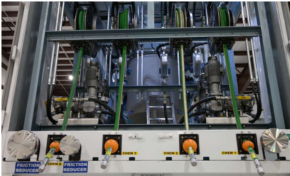
DISCHARGE POLYMER SOLUTION, MANIFOLD
