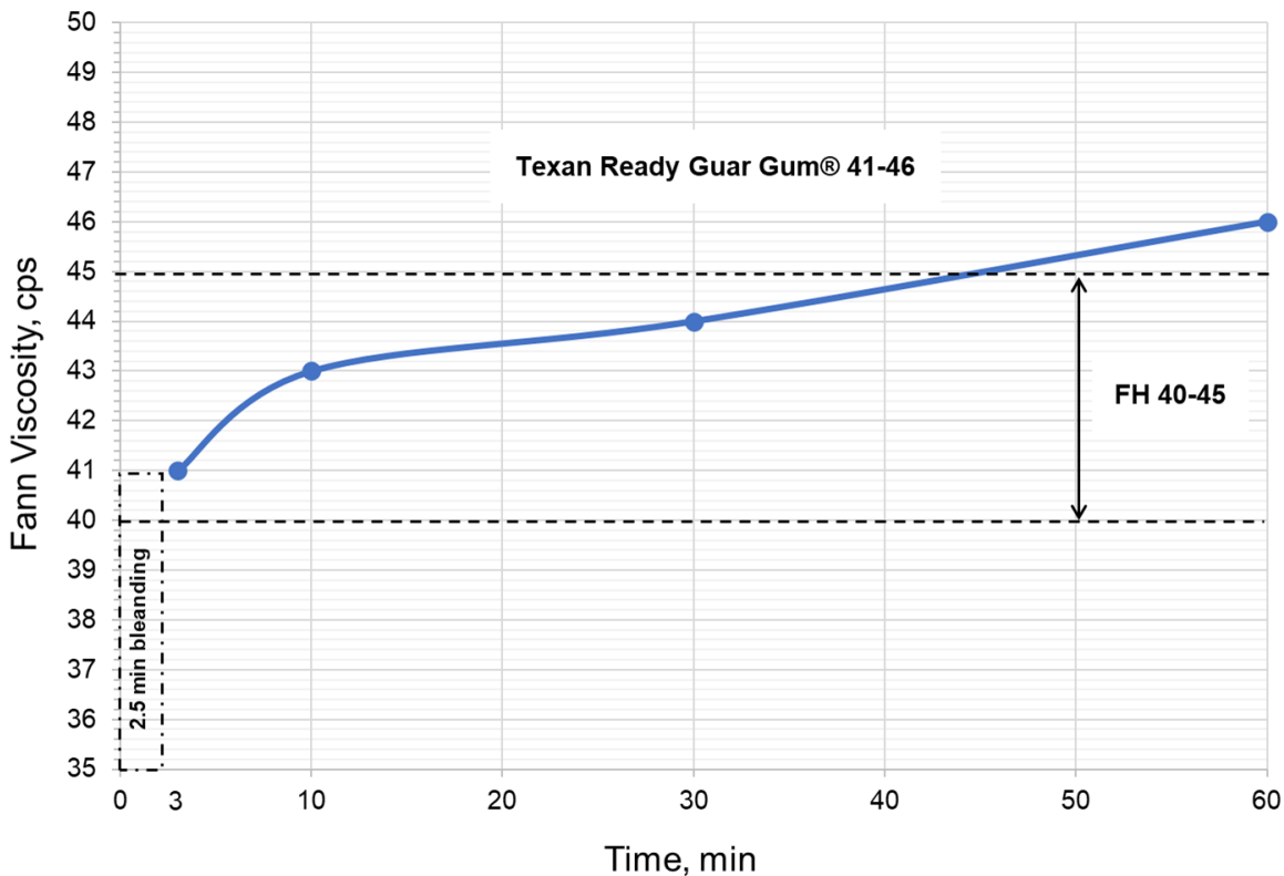
Figure 1. Texan Ready Guar Gum® performance in 2% KCL solution at room temperature
